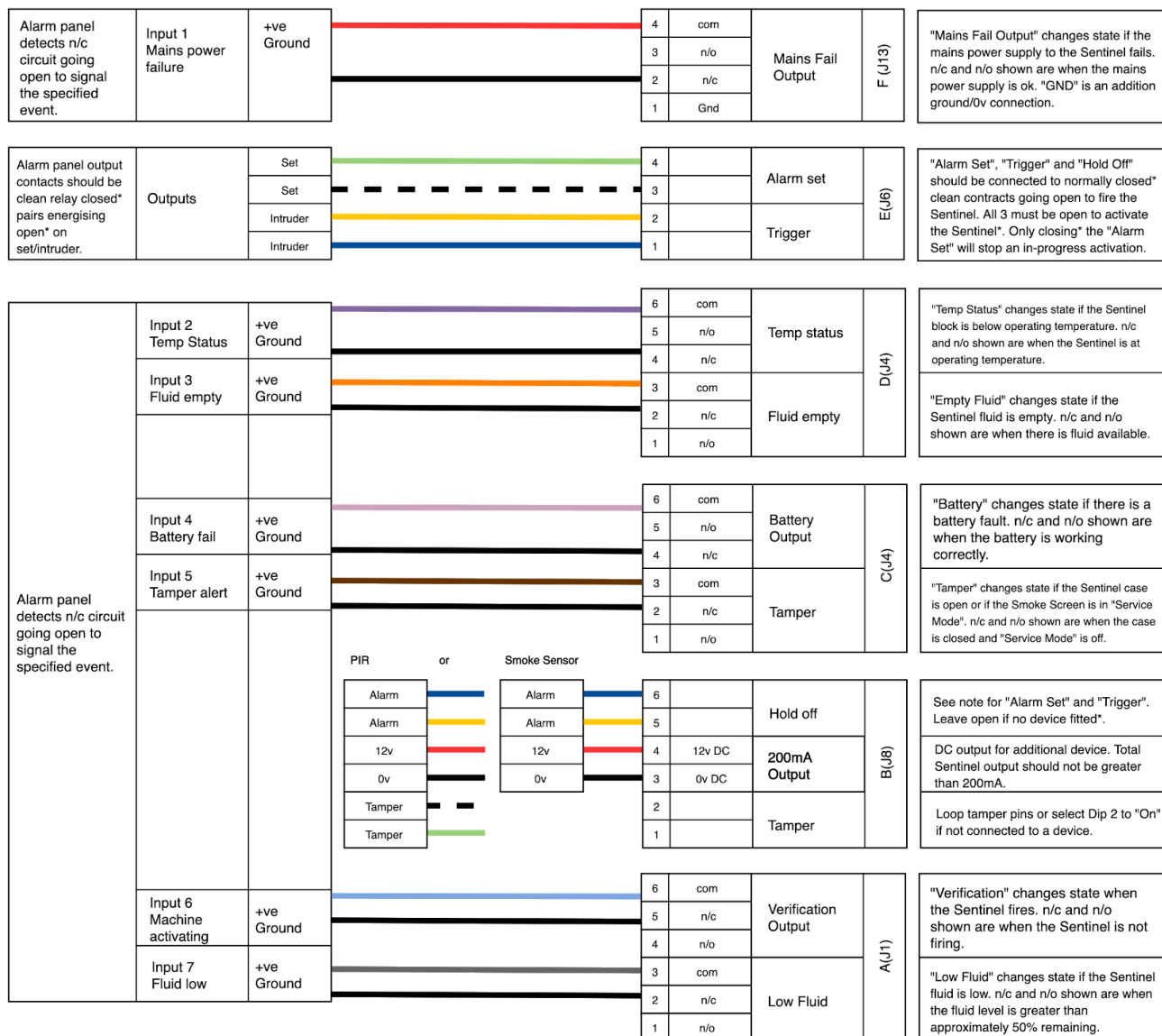
Alarm Panel or similar control device
