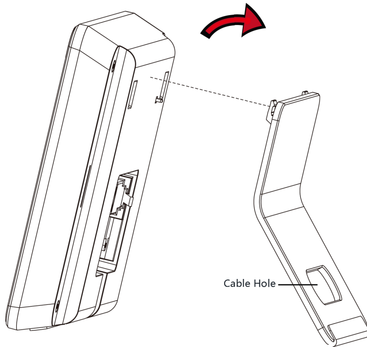
Figure 3-1 Base Mounting
