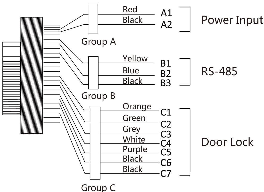
Figure 4-1 Terminal Diagram
