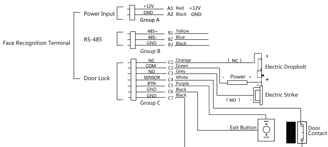
Figure 4-2 Device Wiring
