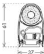
Dimensions CS/STD/RS/1600 – CS/STD/RS/2000 - CS/STD/RSTX/1600 – CS/STD/RSTX/2000
